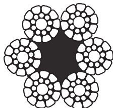
6x19S (9-9-1)
