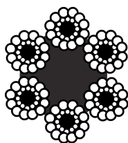
6x24S (12-12-FC)
