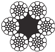
6x26 WS (10-5+5-5-1)
